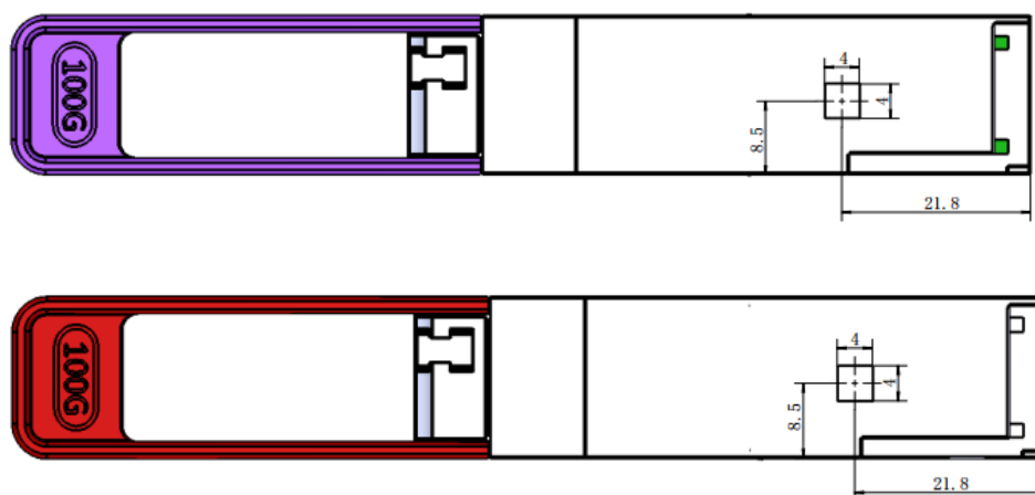
Figure 9: Case Temperature Measurement Point (All dimensions in mm)
