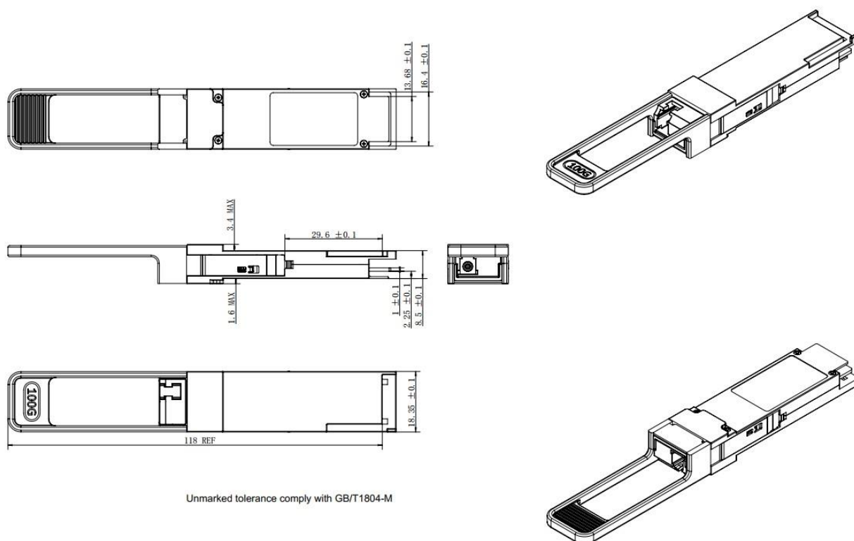
Figure 8: Mechanical Package Outline (All dimensions in mm)
